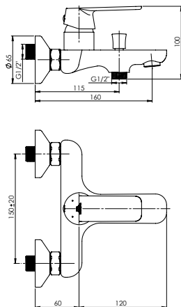
ELMA-10 (K) Bath faucet with shower set | EL10K08
