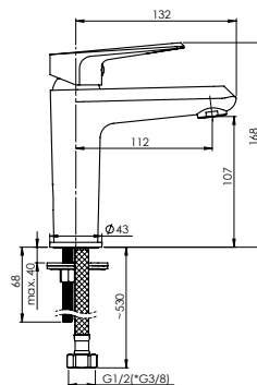
DELI-18 Washbasin faucet | 1/2-D80008 | 3/8-D80108
