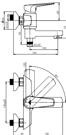
DELI-10 (SW) (K) Bath / shower faucet with shower set | D1PK08
