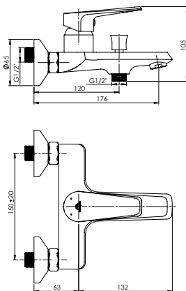
DELI-10 (K) Bath faucet with shower set | D10K08
