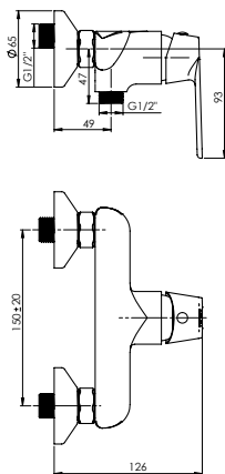
ELMA-12 (K) Shower faucet with shower set | EL20K08
