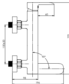
ULTRA-10 (SW) (K) Bath / shower faucet with shower set | U1KP08 | LUX: U1KPL08
