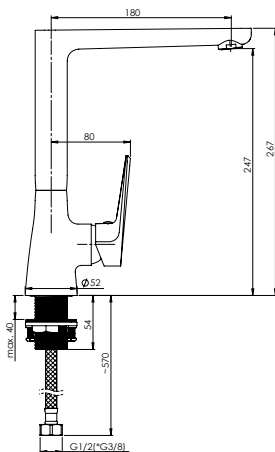
DELI-18 Washbasin faucet | 1/2-D80008 | 3/8-D80108
